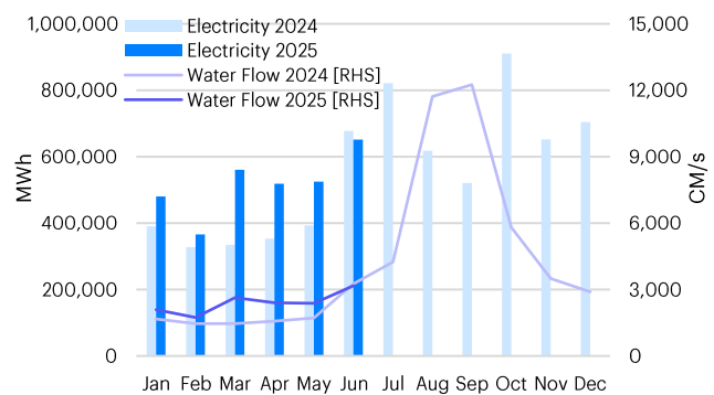
Figure 4: XPCL Water Flow Expected to Higher YoY
