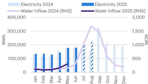
Figure 3: NN2 Electricity in 3Q25F Expected to Grow
