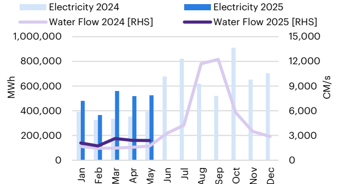
Figure 4: XPCL Water Flow Higher YoY and MoM in May
