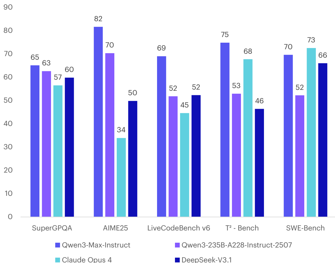
Benchmark performance of Qwen3-max/Qwen3-235B and their counterparts
