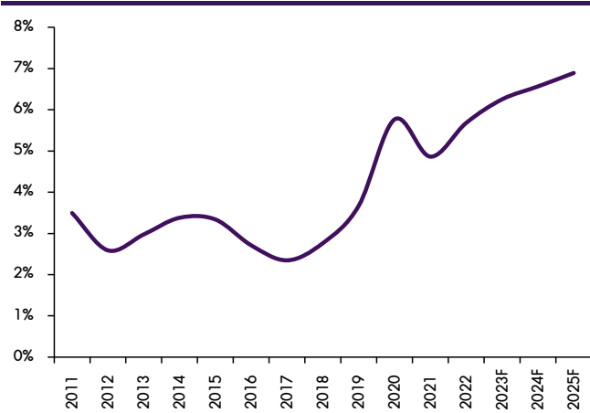
Figure 5: NPL ratio
