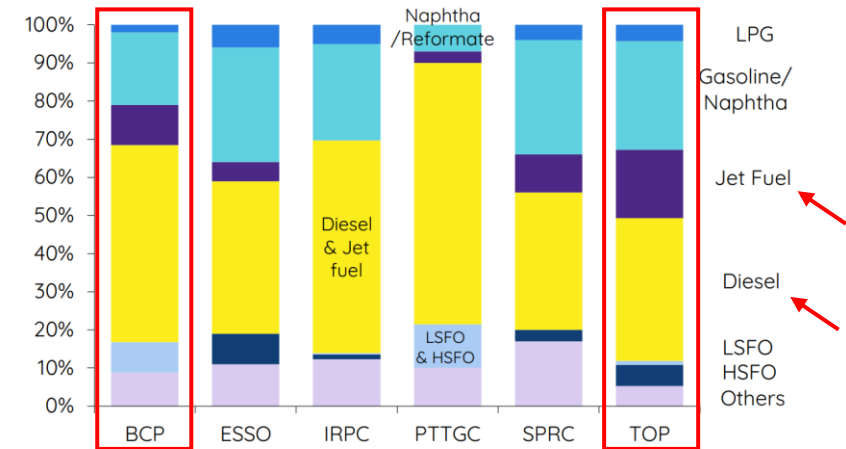
Figure 8: BCP Having High Diesel Yield, While TOP Having High Jet Fuel
